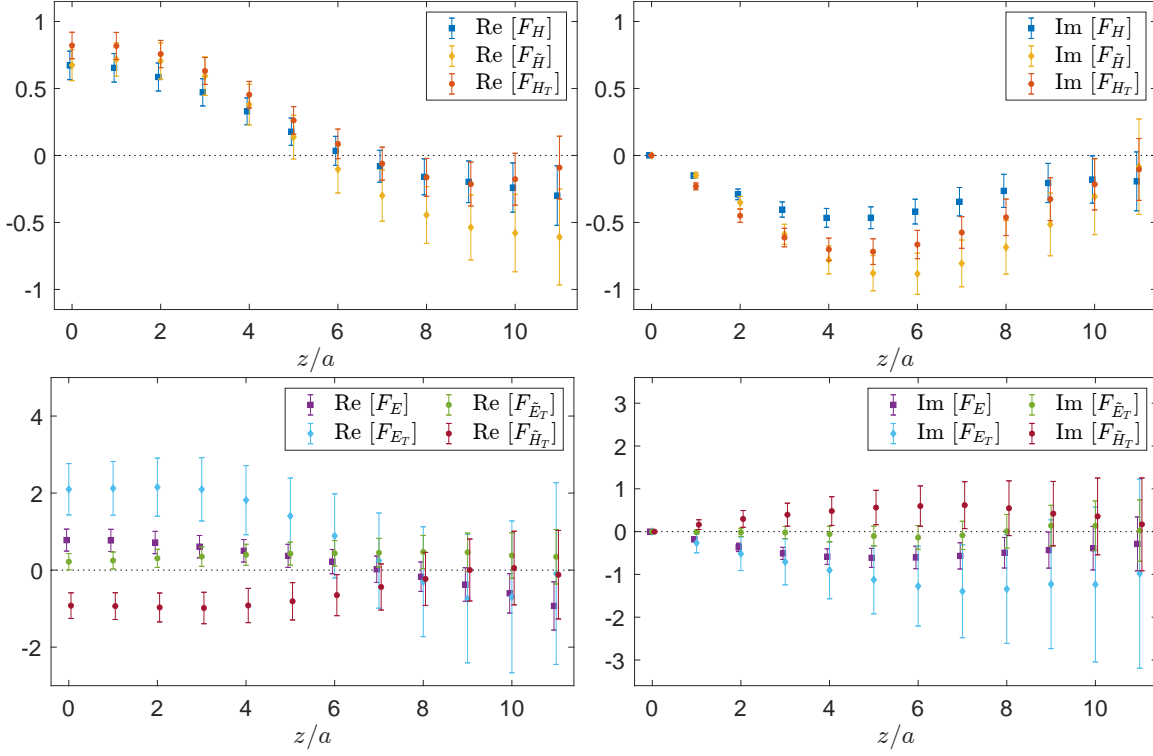
Figure 1: Real (left) and imaginary (part) part of the matrix elements for the leading (top) and subleading GPDs (bottom) at \{P_3 = 1.67, \xi = 0, -t = 0.69 \text{ GeV}^2\} . Data are renormalized in a variant of the RI-MOM scheme at (a\mu_0)^2 \approx 2.57 .
