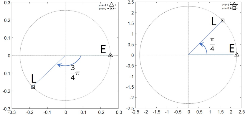
Figure 1: We plot the expectation values of \frac{1}{N} \text{Tr} A_0^2 (Left), and \frac{1}{N} \text{Tr} A_i^2 (Right). Those of the Euclidean model are represented by the triangle and the letter “E”, and those of the Lorentzian model are represented by the square and the letter “L”. The angle between \langle \frac{1}{N} \text{Tr} \tilde{A}_0^2 \rangle_E and \langle \frac{1}{N} \text{Tr} A_0^2 \rangle_L is -3\pi/4 , in agreement with Eq. (10), and the angle between \langle \frac{1}{N} \text{Tr} \tilde{A}_i^2 \rangle_E and \langle \frac{1}{N} \text{Tr} A_i^2 \rangle_L is \pi/4 , in agreement with Eq. (11).
