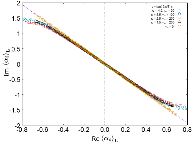
Figure 2: Expectation values of the eigenvalues \alpha_i of A_0 for N = 128 . The \gamma_\alpha = 0 case (inverted triangles) corresponds to the Euclidean model, where the complex phase of the expectation values \langle \alpha_i \rangle_L is \exp(-i3\pi/8) . Those points lie, as expected, on the purple line. When (\kappa, \gamma_\alpha) = (4.5, 50) , (3.5, 100) , (2.5, 200) , (1.5, 200) , we obtain the curves that go through the circles, the squares, and the triangles, respectively. The points near zero lie on the purple line, which implies that the emergent time is Euclidean. On the other hand, as we move further from zero, we obtain almost real (\Delta\alpha_i)_L , which implies the emergence of Lorentzian time.
