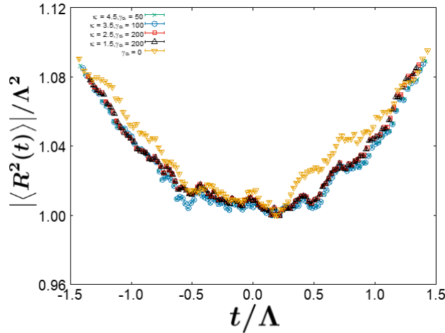
Figure 4: |\langle R^2(t) \rangle|/\Lambda^2 is plotted against t/\Lambda for N = 128 and (\kappa, \gamma_\alpha) = (4.5, 50), (3.5, 100), (2.5, 200), (1.5, 200) , where \Lambda = |\langle R^2(0) \rangle|^{1/2} . The symbols are the same as in Fig. 2. We observe scaling behavior and a slight expansion of space as t/\Lambda moves away from zero.
