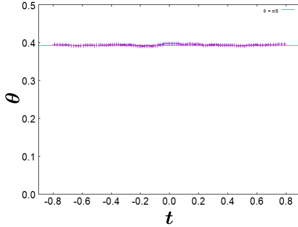
Figure 3: \theta(t) is plotted against t for N = 128 and (\kappa, \gamma_\alpha) = (4.5, 50) . All values of \theta(t) are on the \theta = \pi/8 line, which implies that the emergent space is Euclidean.
