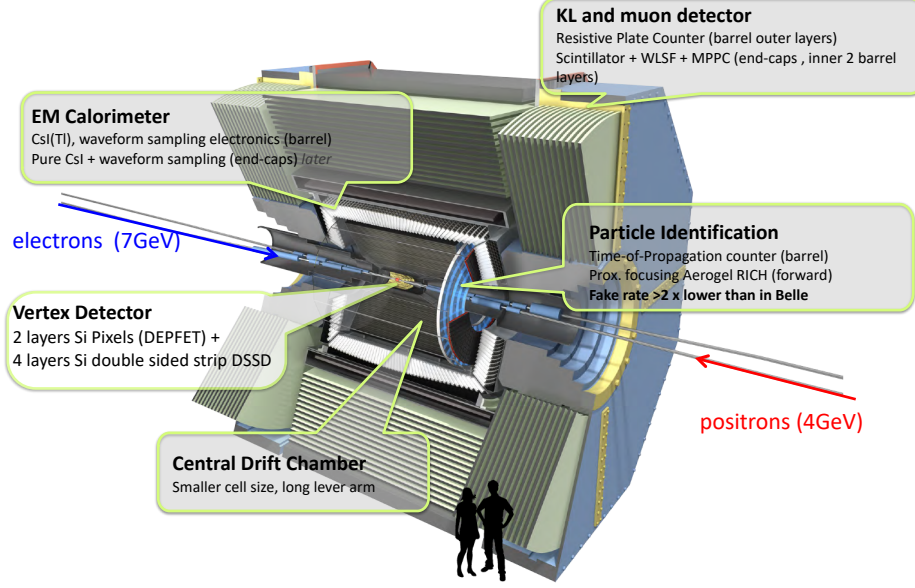
Figure 1: Schematic of the Belle II detector [2].
