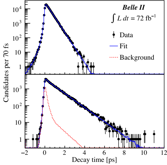
Figure 3: Decay-time distributions of (top) D^0 \rightarrow K^- \pi^+ and (bottom) D^+ \rightarrow K^- \pi^+ \pi^+ candidates in their respective signal regions with fit projections overlaid [4].
