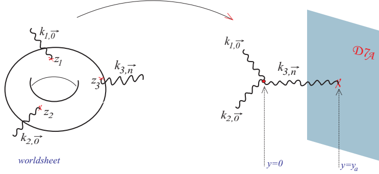
Figure 2: Non-zero contribution from 1-loop; 3-graviton scattering amplitude of 2 massless gravitons and 1 KK mode corresponding to a closed string propagation in 2-dimensions towards a D7 brane.
