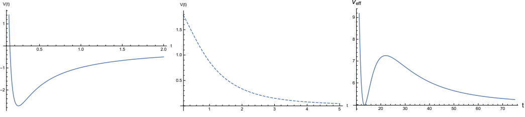
Figure 1: Left figure: Vanishing of V(\tau) from 0^- happens for potentials with an AdS minimum. Middle: Large \tau behaviour of V(\tau) with power law correction \sim \frac{1}{\tau^\pi} . The potential on the right-hand side exhibits local minimum and maximum.
