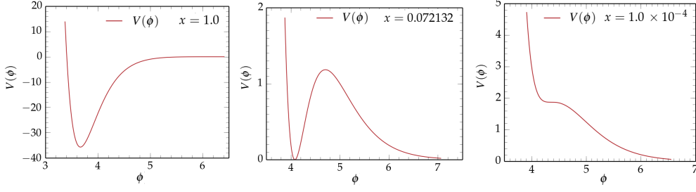
Figure 3: Scalar potential V(\phi) for different values of x giving an AdS, Minkowski or dS vacuum.
