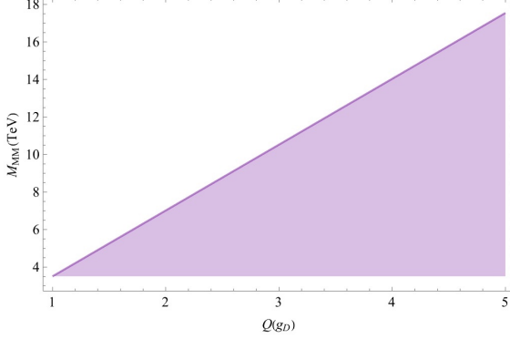
Figure 2: Exclusion limits (purple region) on MM mass as a function of Q in Dirac charge g_D units, by using limits on \zeta_{1,2}^Y [7].
