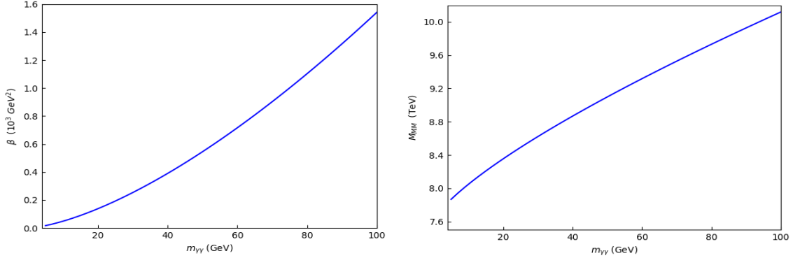
Figure 3: Born-Infeld parameter \beta (left) and MM mass \mathcal{M}_{MM} (right) limits versus m_{\gamma\gamma} in Pb-Pb collisions by using ATLAS and CMS data [4, 5].
