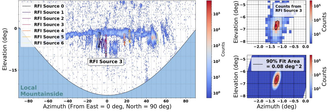
Figure 4: Left: 2D histogram of events from one week in September 2021. Seven of the most populated RFI sources have been highlighted. Top Right: Isolated events from RFI Source 3. Bottom Right: 2D Gaussian fit (color map), with the outline of the 90% integral area. The average fit 90% integral area for all 7 sources was < 0.1 sq. degrees. Figure sourced from [7].
