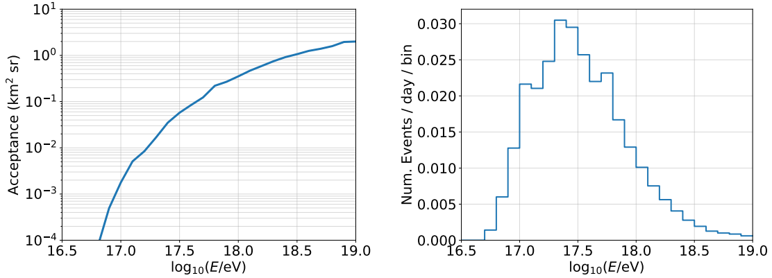
Figure 3: Left: The acceptance ( \text{km}^2 \text{sr} ) of the BEACON prototype array to cosmic arrays as a function of cosmic ray energy for a power-SNR threshold of 10. Right: The expected number of cosmic ray events per day as a function of energy assuming the cosmic ray flux measured by Auger [11]. \sim 0.3 events per day are expected total.
