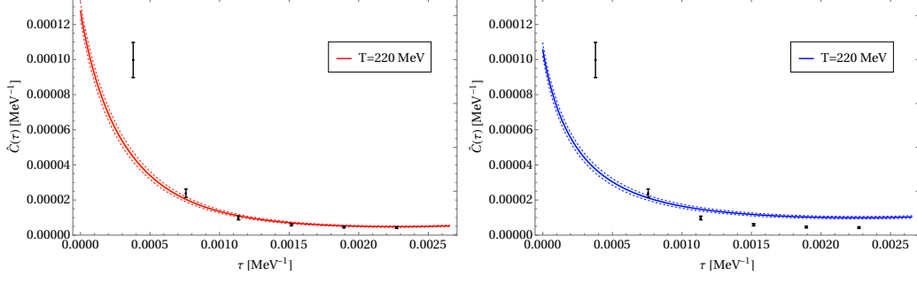
Figure 7: Left: Temporal correlation function predicted by the spectral function Eq. (12), Fig. 6 (red band), compared to the full lattice data from Fig. 2 [5]. Right: The corresponding prediction based on a Breit-Wigner ansatz, Eq. (13).
