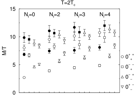
Figure 3: Screening masses computed within EQCD, after integrating out N_f massless fermions. Filled symbols correspond to operators constructed from colour-magnetic fields exclusively, \text{Tr}F_{ij}^2, \dots , open symbols contain colour-electric fields \text{Tr}(A_0^2), \text{Tr}(A_0 F_{ij}), \dots . From [8].
