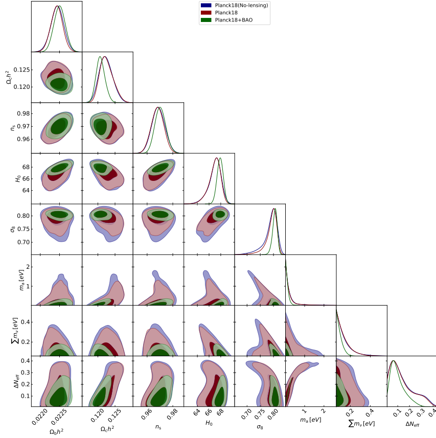
Figure 7: Allowed regions and one-dimensional probability posterior distributions for the KSVZ axion (figure from Ref. [28]).
