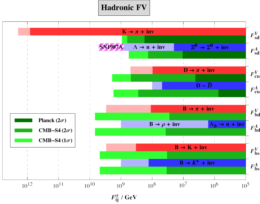
Figure 5: Current bounds and future prospects for flavor-violating axion interactions with quarks (figure from Ref. [27]).
