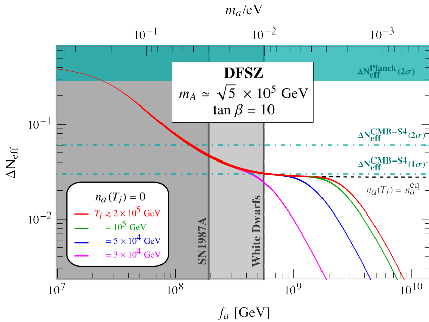
Figure 4: \Delta N_{\text{eff}} as a function of the axion decay constant for the DFSZ axion (from Ref. [25]).
