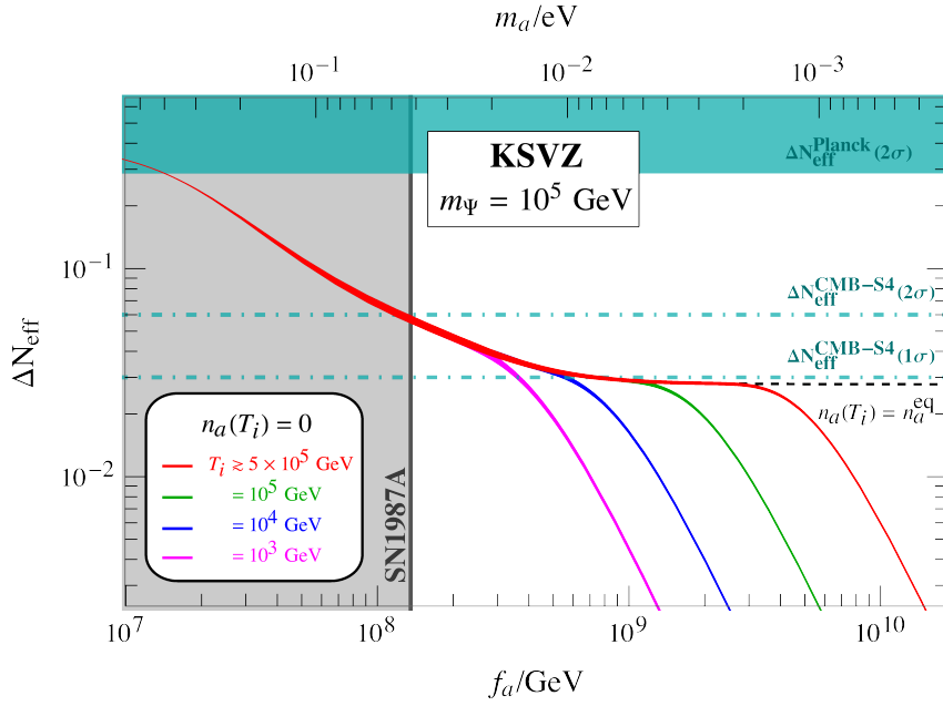
Figure 3: \Delta N_{\text{eff}} as a function of the axion decay constant for the KSVZ axion (from Ref. [25]).
