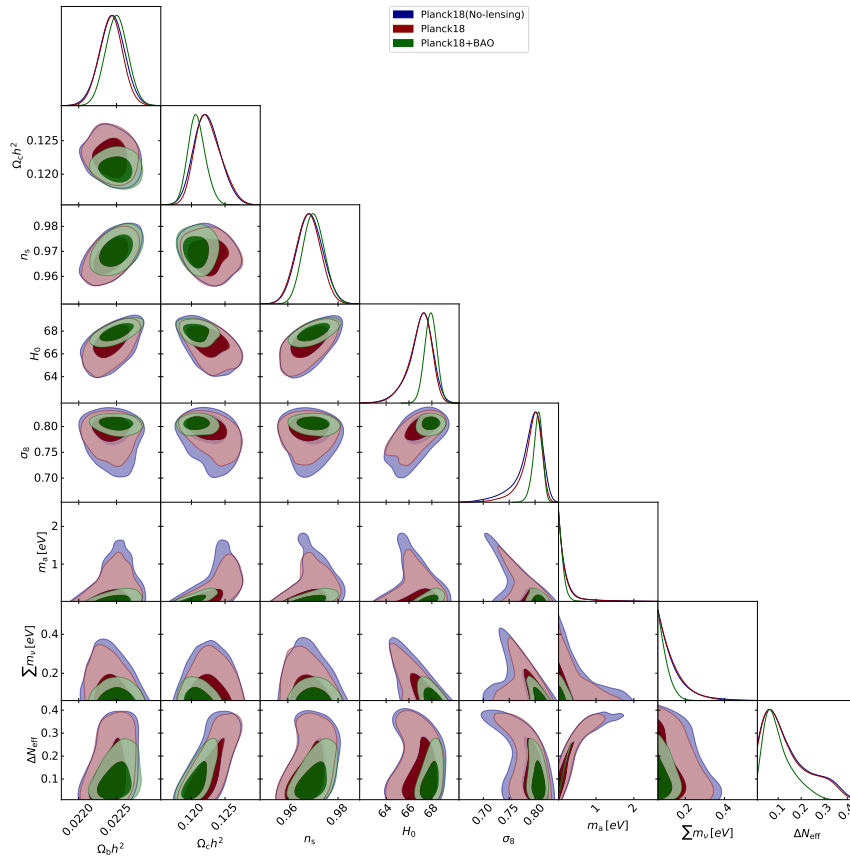
Figure 8: Allowed regions and one-dimensional probability posterior distributions for the DFSZ axion (figure from Ref. [28]).
