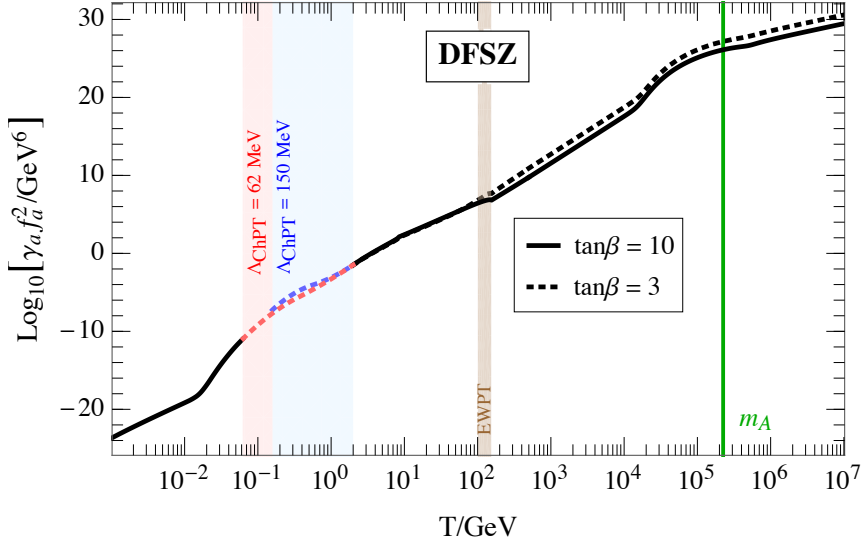
Figure 2: Production rate as a function of the temperature for the DFSZ axion (from Ref. [25]).
