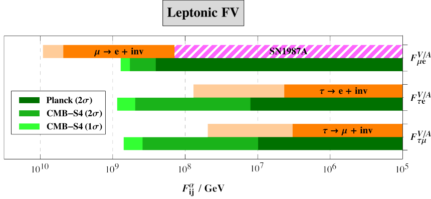
Figure 6: Current bounds and future prospects for flavor-violating axion interactions with leptons (figure from Ref. [27]).
