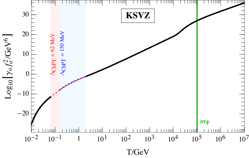
Figure 1: Production rate as a function of the temperature for the KSVZ axion (from Ref. [25]).
