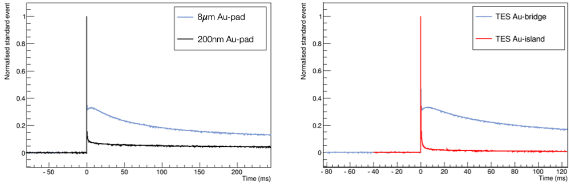
Figure 3: A comparison of pulse shapes of particle interactions directly in the Au-pad. Left: A comparison between pulse shapes of detectors having different Au-pad thickness read out with the TES bridge design; Right: Pulse shapes of detectors having different TES designs.
