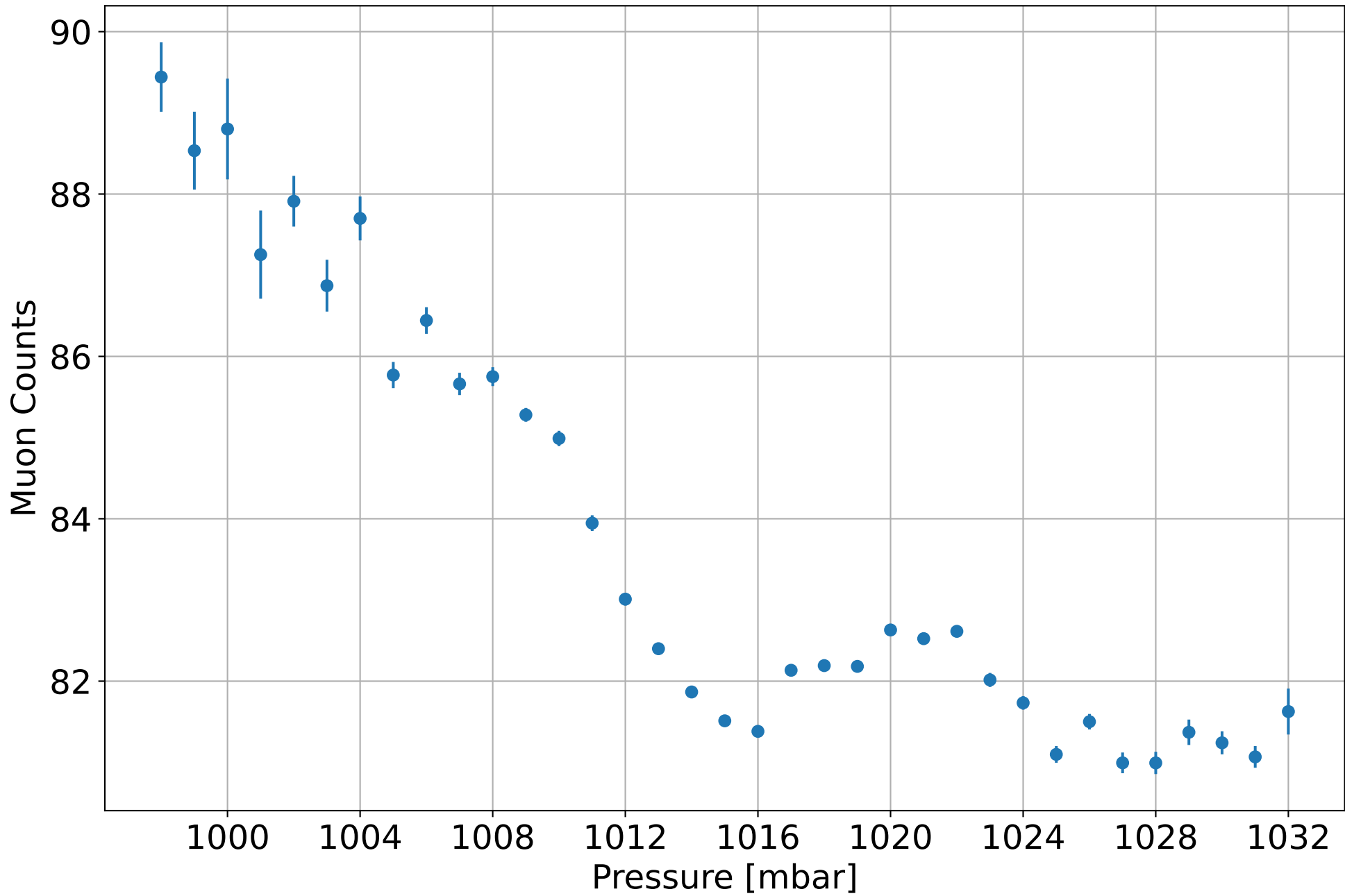
Muon counts vs Pressure - Correlation:-0.916+/-0.070
