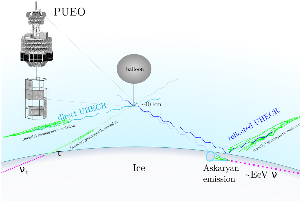
Figure 1: A diagram of the PUEO instrument and the types of radio emission from particles it will be capable of detecting. The direction, frequency content, polarity and polarization of the pulses differentiate the types of pulses.
