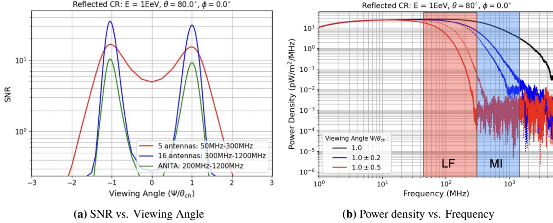
Figure 2: Left: The SNR of a simulated reflected cosmic ray event as a function of viewing angle (relative to the Cherenkov angle \theta_{ch} \sim 0.6^\circ ) for different frequency bands. Right: the power spectral density of a simulated reflected cosmic ray event. Targeting the lowest frequency range of 50-300 MHz will have the best chance of seeing a reflected cosmic ray event as the SNR is high across a large range of view angles.
