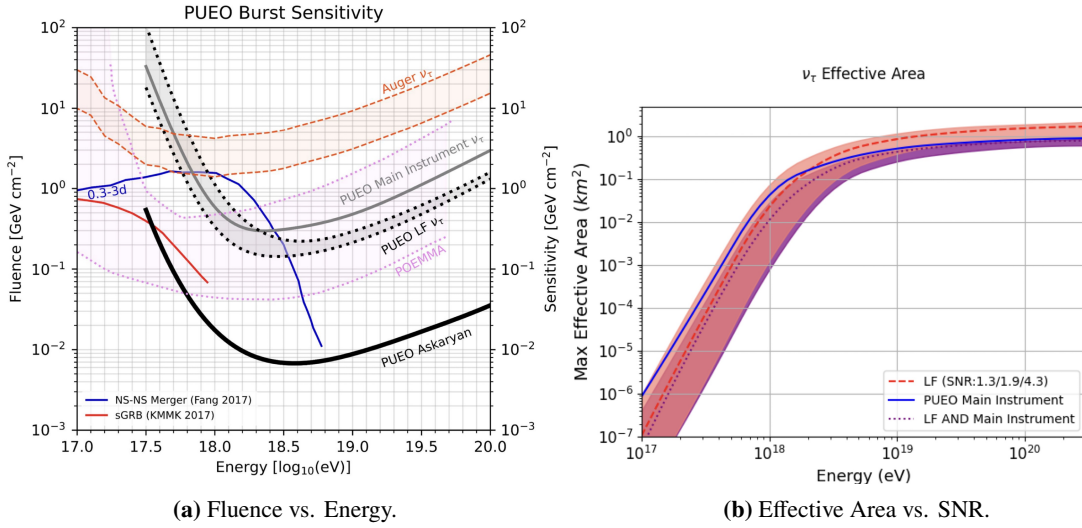
Figure 6: Left: the fluence of the PUEO instrument in response to a burst event of length 0.3-3 days, compared to other experiments. Right: The \nu_\tau effective area as a function of \nu_\tau energy.
