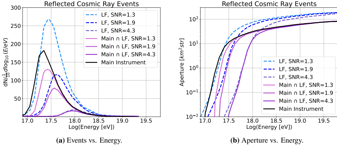
Figure 5: Left: the number of reflected cosmic ray events seen by each of PUEO’s instruments as a function of primary energy. The different line styles are three possible thresholds for the LF instrument. Right: The aperture of the PUEO instruments as a function of reflected cosmic ray energy.
