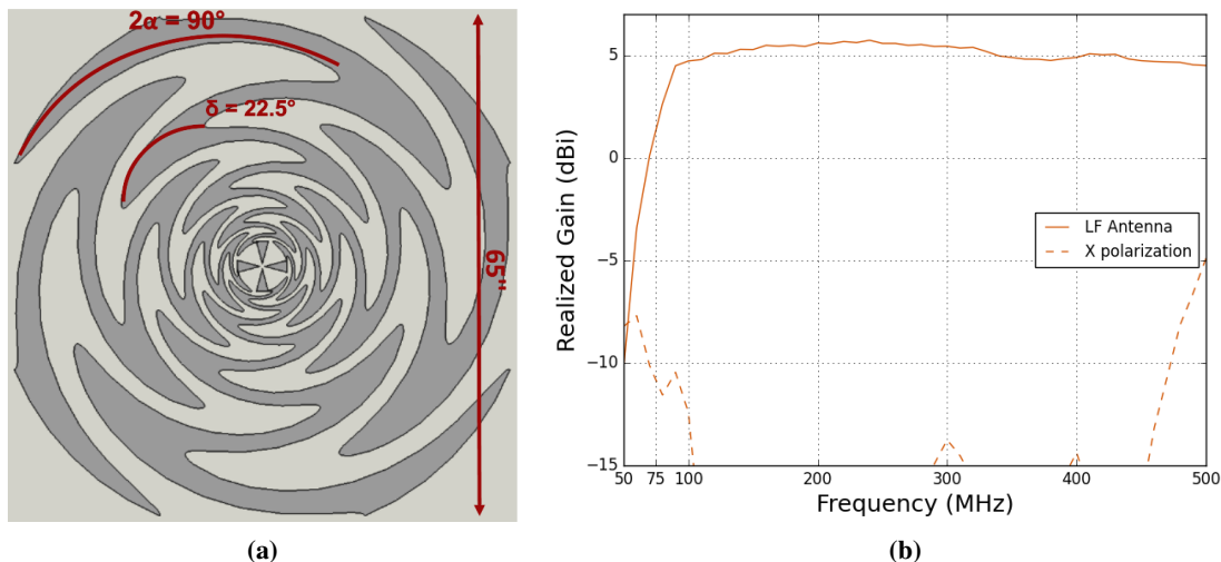
Figure 4: Left: A close up of the LF sinuous antenna. Right: a plot of the frequency response of the LF antenna. The response is fairly uniform across the 90-500 MHz band.
