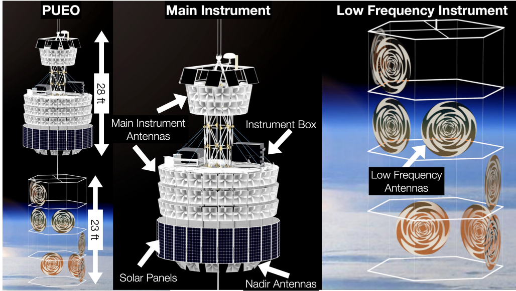
Figure 3: A diagram showing the PUEO instrument. Left panel: the full instrument as it will be deployed. Middle: the main instrument, including the instrument box and 108 broadband dual polarized antennas. Right panel: The Low Frequency instrument, with 8 dual-polarized broadband antennas.
