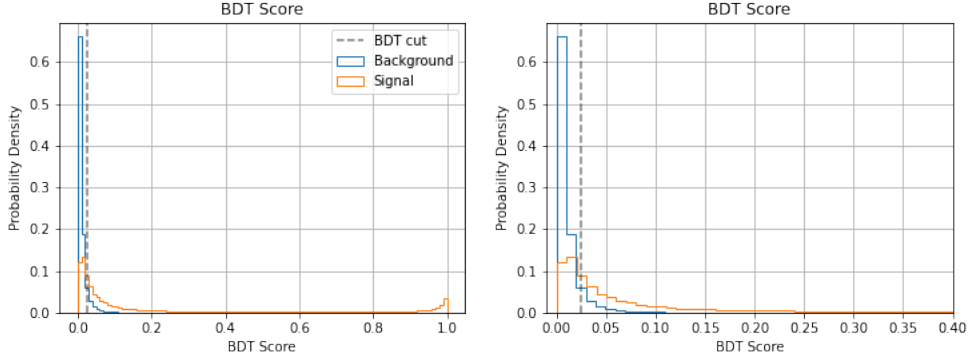
Figure 1: These plots show the distribution of BDT scores for background and signal events. The right plot is a zoomed-in plot of the left. The score, ranging from 0 to 1, indicates the probability of an event being a background versus signal (0 being more background-like and 1 being more signal-like).
