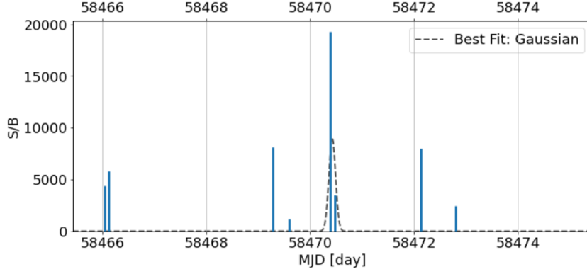
Figure 4: This is a time series plot near the best fit flare. The events are shown as blue lines. The heights of the lines indicate the ratio between the signal probability (Equation 3) and the background probability (Equation 5) of each event. The x-axis shows MJD in days. The dashed black curve is the best fit Gaussian flare with a mean at T_0 = 58470.42 and a width of \sigma_T = 0.063 . The height of the curve is arbitrary.
