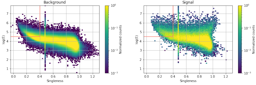
Figure 3: These two plots are 2D histograms of the singleness predicted by the BDT regressor versus energy. The left plot shows background distribution and the right shows signal. Events in the upper left corner ( \log_{10} E > 4.5 and singleness < 0.4 ) are removed from the dataset.
