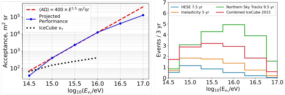
Figure 3: Left: IceCube and projected TAMBO \nu_\tau acceptance as functions of energy assuming 22,000 cubic-meter-sized water Cherenkov detectors arranged with 150 m separation on a triangular grid, adapted from Ref. [17]. Right: Projected number of events observed by TAMBO given the acceptance shown in the left panel under different flux model assumptions [6, 18–20].
