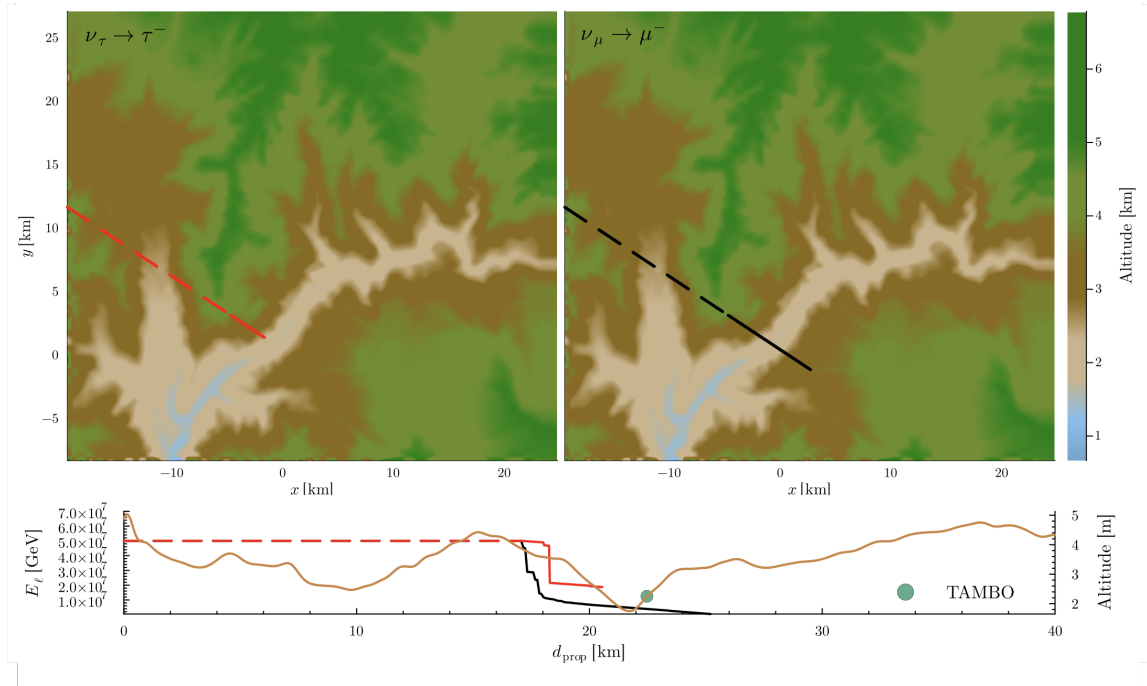
Figure 4: Simulation of a tau (solid red) and muon (solid black) and their parent neutrinos (dashed) passing through the Colca Canyon geography near TAMBO. The top two panels illustrate the complex geometry of the canyon and surrounding mountains, which is fully implemented in the simulation, and the path taken by the aforementioned leptons. The bottom panel shows the leptons' energies as they travel through the geography near the canyon, and a cross section of the canyon profile (brown).
