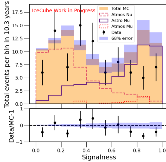
Figure 6: Data vs Monte Carlo comparison for the signalness evaluated by Eq. 2. The MC over predicts the data substantially in 3 signalness bins, a direct propagation of the data/MC mismatch seen in Fig. 2. Work is in progress to resolve this.
