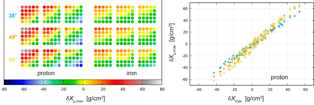
Figure 5: Left: relative change of X_{\mu,\max} for r > 1000 m. Right: correlation with mean X_{\max} shift for primary protons; different colors indicate different zenith angles, with colors indicated on the left panel.
