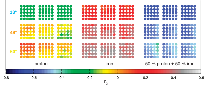
Figure 8: Ranking coefficient r_G for S_\mu(1000) – X_{\max} correlation for proton, iron and mixed primary beams for the three zenith angles where full X_{\max} coverage is available.
