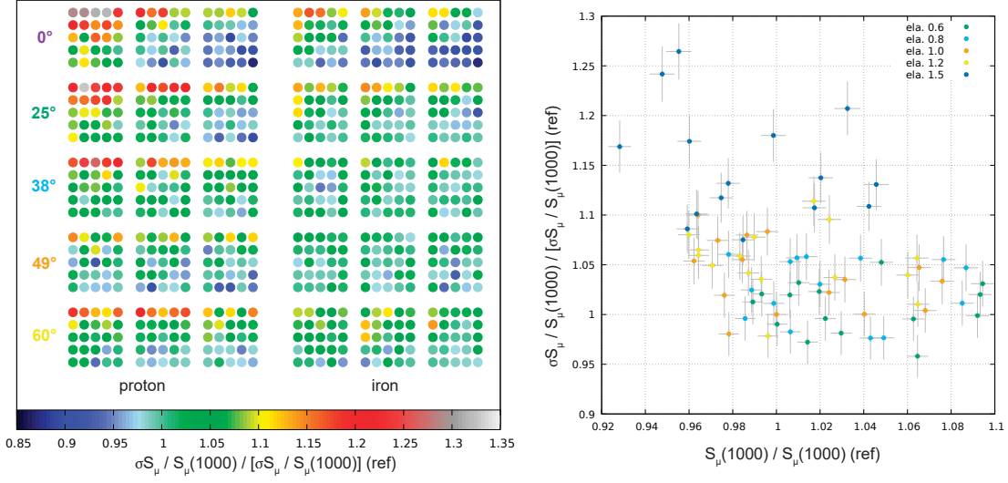
Figure 7: Left: relative change of relative fluctuations of muon signal at 1000 m for all relevant bins. Right: correlation with the relative change of in S_\mu(1000) for primary protons for \theta = 38 ; different colors indicate different change of elasticity.
