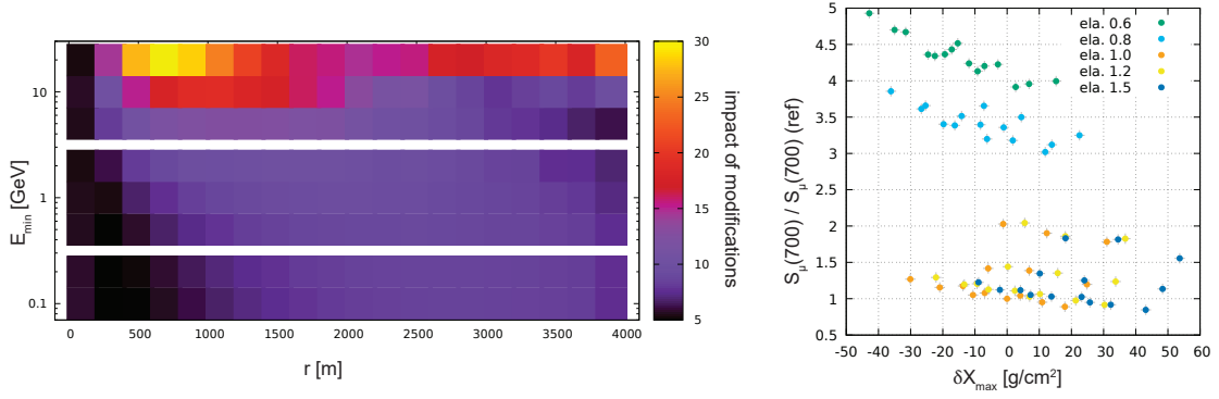
Figure 9: Left: impact of modifications on muon densities for different radial distance and E_{\min} . Right: S_\mu – X_{\max} plot for the most significant combination, colored by elasticity.
