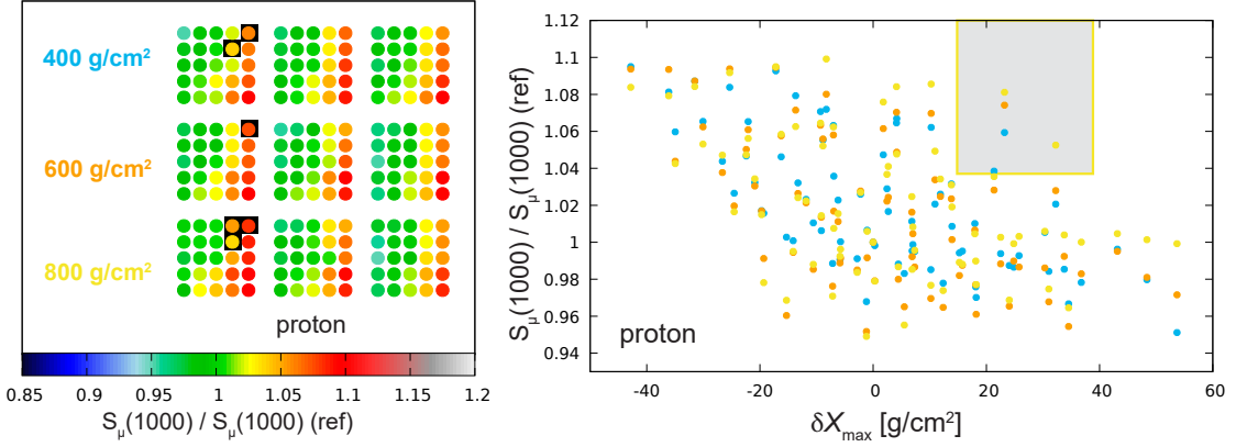
Figure 6: Left: relative change of muon signal at 1000 m for three different distances between the ground and the shower maximum DX. Right: correlation with mean X_{\max} shift for primary protons; different colors indicate different DX, with colors indicated on the left panel; the shaded area corresponds to the results of the Pierre Auger Observatory at \theta = 55^\circ [6] and the modifications that fall within this area are highlighted in the left panel.
