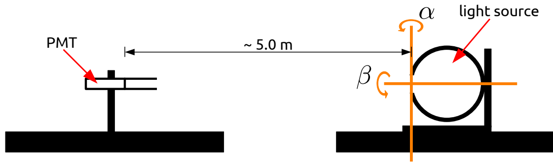
Figure 2: Schematics of the laboratory setup to characterize the angular emission of the light sources.
