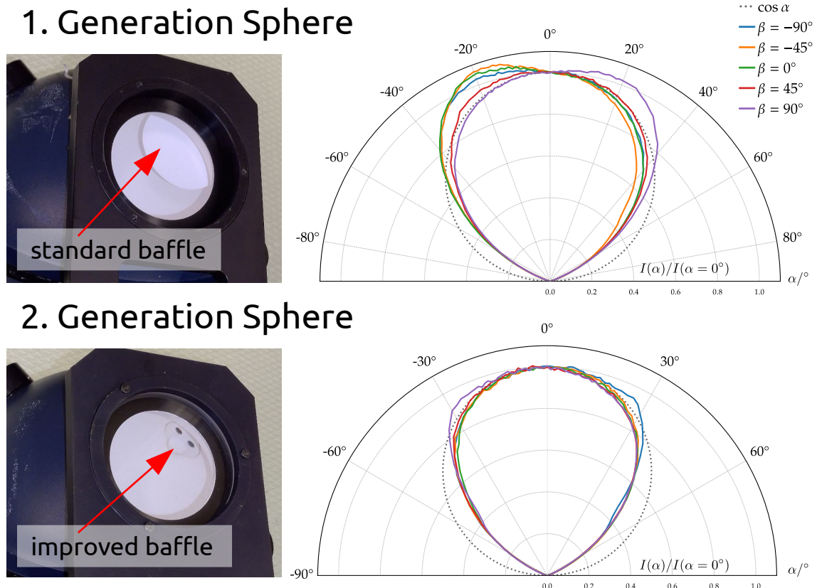
Figure 3: Measurements of the angular emission characteristics of the two generations of integrating-sphere light sources.
