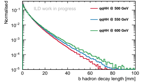
Figure 2: Decay lengths of weakly decaying b -hadrons, comparing 500 GeV, 550 GeV and 600 GeV.
