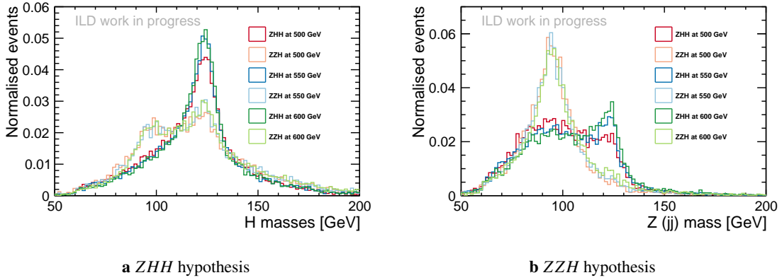
Figure 3: Di-jet masses using the pairing according to a ZHH hypothesis and a ZZH hypothesis, comparing ZHH and ZZH events at 500, 550 and 600 GeV.
