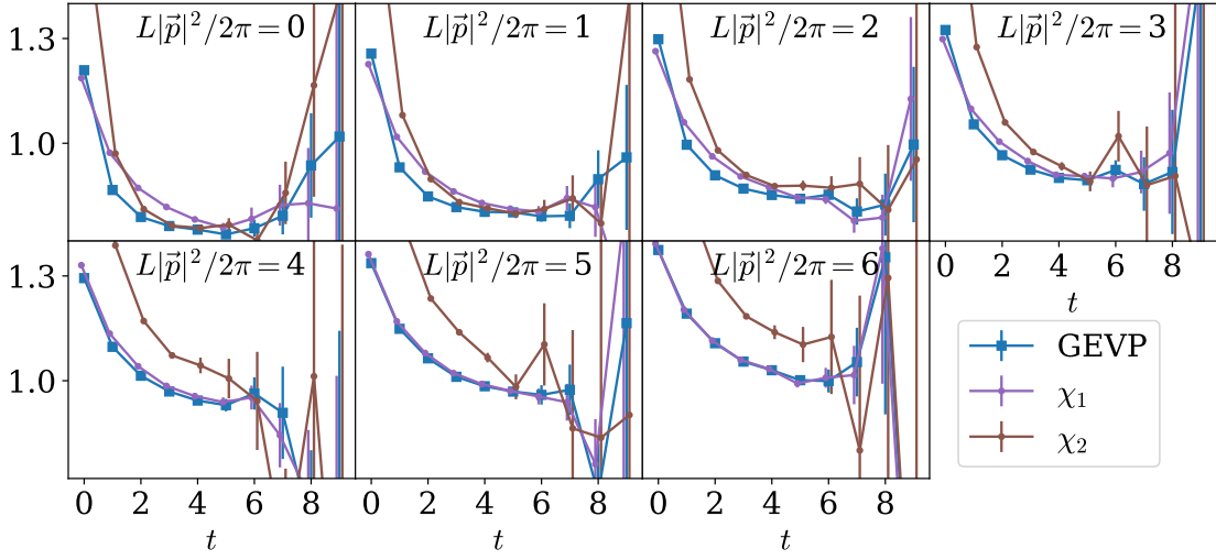
Figure 1: Effective energies E_{\text{eff}}(t) = \log(C^{2\text{pt}}(t)/C^{2\text{pt}}(t+1)) as a function of sink time t for the different boost momenta, comparing the diagonal correlators C_{ii}^{2\text{pt}} of Eq. (9) computed with single interpolators from the basis Eq. (2) with the GEVP-optimized one of Eq. (11) defined with the composite interpolator Eq. (10)
