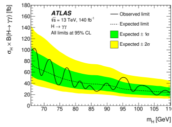
Figure 6: 95% CL upper limit on \sigma_S \times \mathcal{B} versus mass of the low-mass Higgs boson [6].
