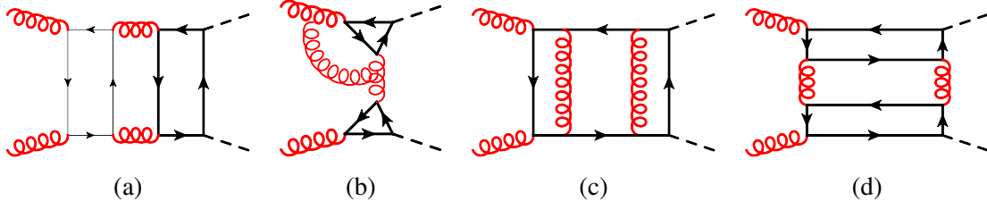
Figure 1: Classification of the three-loop virtual corrections to gg \rightarrow HH .
