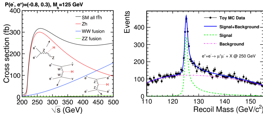
Figure 1: Higgs production at the ILC. Left: cross sections for the three major production processes as a function collision energy [6]. Right: recoil mass spectrum for signal of Higgs boson production and SM background at 250 GeV ILC, for Z \rightarrow \mu^+\mu^- selection [7].
