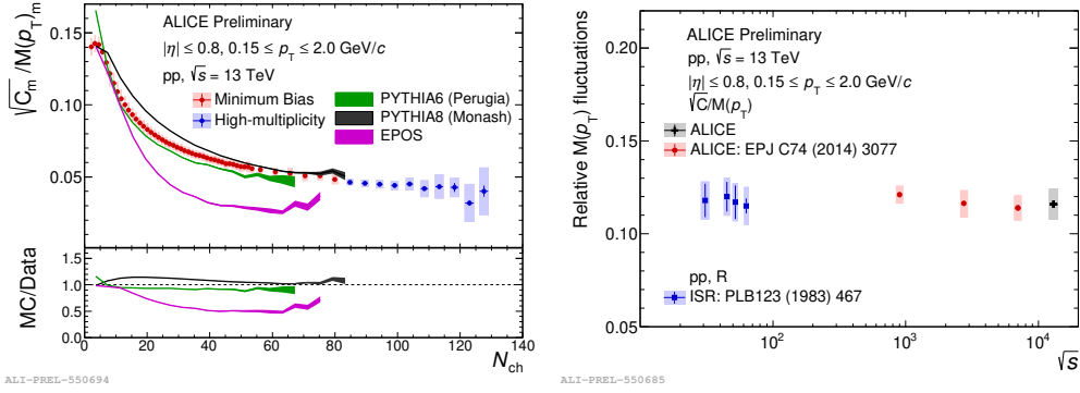
Figure 2: Models predictions compared with the experimental findings (left). Inclusive correlator values from ISR to LHC energies (right). The statistical errors are represented by lines and systematic errors by shaded boxes.
