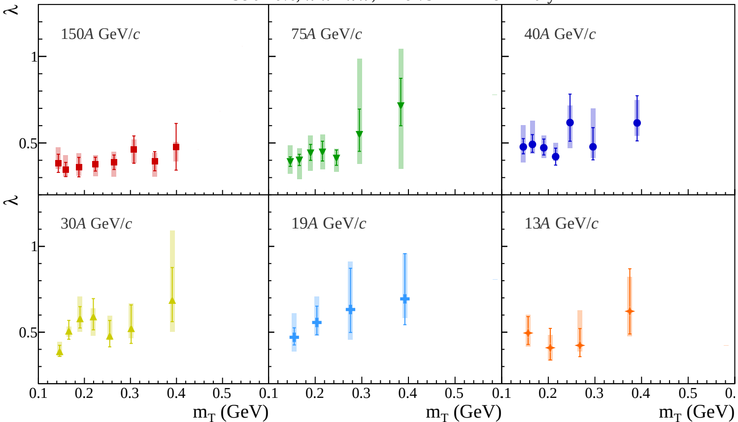
Ar+Sc 0-10%, \pi^+\pi^+\pi^-\pi^- , NA61/SHINE Preliminary
