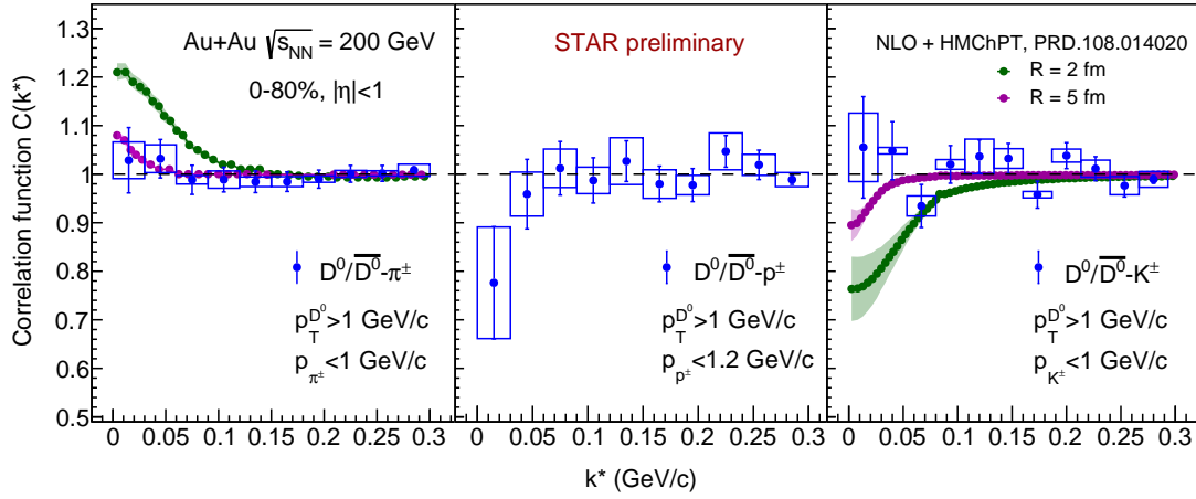
Figure 2: Femtoscopic correlation functions between D^0/\overline{D}^0 mesons and \pi^\pm (left panel), p^\pm (middle panel) and K^\pm (right panel) pairs obtained for Au+Au collisions at \sqrt{s_{NN}} = 200 GeV with |\eta| < 1 . Blue solid points represent experimental data. They are shown with statistical and systematic (marked with boxes) uncertainties. In the case of D^0/\overline{D}^0 - \pi^\pm and D^0/\overline{D}^0 - K^\pm , the experimental data are compared with theoretical model predictions from [14] for source size of 2 fm (green band) and 5 fm (pink band).
