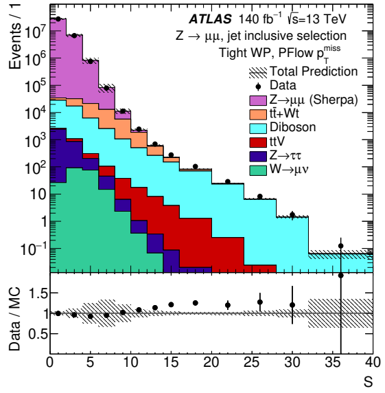
Figure 5: Object-based significance of p_T^{\text{miss}} in Z^0 \rightarrow \mu^+\mu^- events [13].
