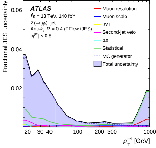
Figure 1: Systematic uncertainty in the MPF response ratios as a function of the reference p_T ( p_T^{\text{ref}} ) for jets calibrated up to, and including, the \eta intercalibration for Z^0(\rightarrow \mu^+ \mu^-) + \text{jet} events [11].
