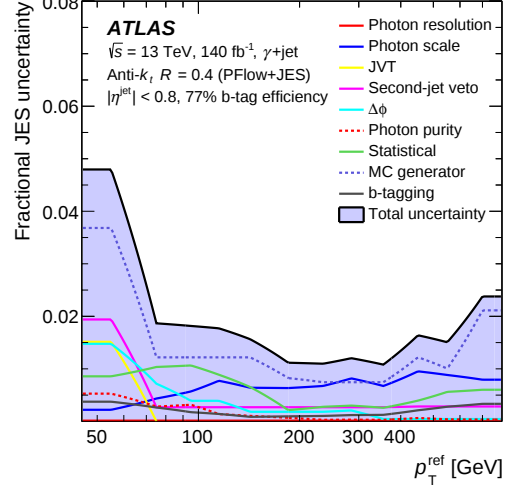
Figure 2: Summaries of uncertainties in the MC-to-data response ratio as a function of p_T^{\text{ref}} for \gamma + \text{b-tagged jet} events [11].
