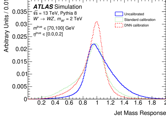
Figure 3: Boosted W/Z-mass response for different calibrations [12].
