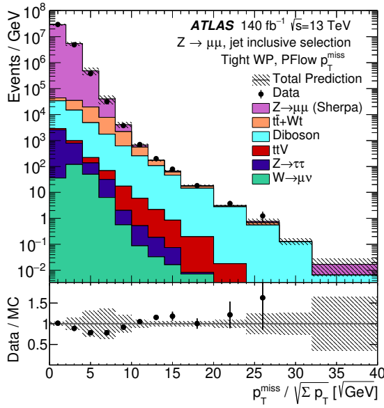
Figure 4: Event-based proxy for p_T^{\text{miss}} significance in Z^0 \rightarrow \mu^+\mu^- events [13].
