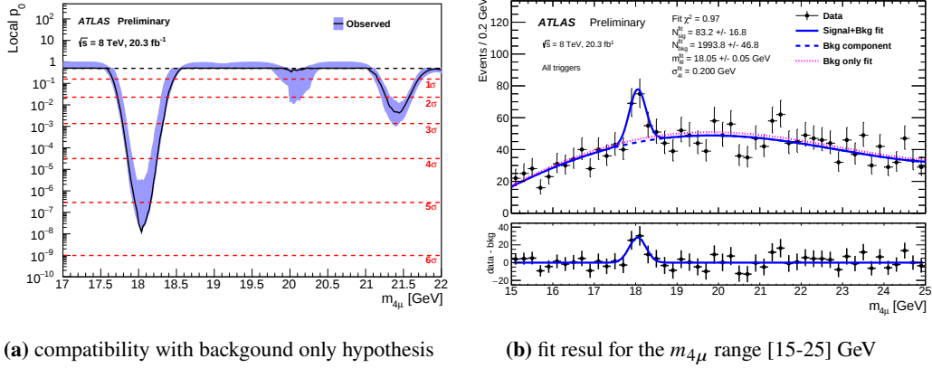
Figure 2: Statistical results for analysis of \sqrt{s} = 8 TeV data from [13]
