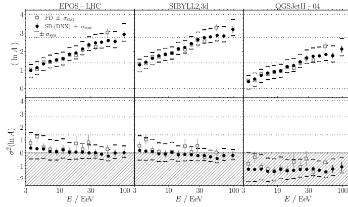
Figure 7: Mean and variance of the logarithm of the mass number \ln A inferred from the SD X_{\max} using different hadronic models.
