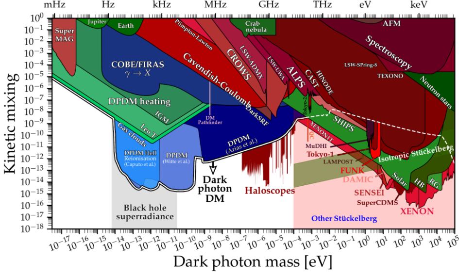
Figure 1: Hidden photon DM parameter space.
