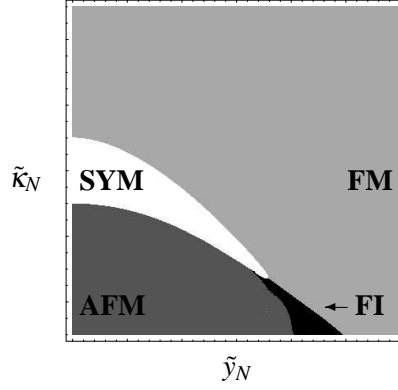
Figure 1: Qualitative phase diagram with respect to the Yukawa coupling \tilde{y}_N and the hopping parameter \tilde{\kappa}_N for a constant quartic coupling \tilde{\lambda}_N = 0.1 .
