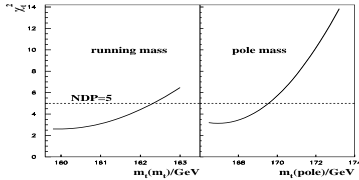
Figure 2: The \chi^2 profile for the Tevatron and LHC t\bar{t} cross section data [9, 10] versus the t -quark mass obtained in the variants of ABM12 fit with those data included and different t -quark mass definitions (running mass: left, pole mass: right). The NDP = 5 for this subset is displayed by the dashed line.
