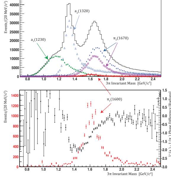
Figure 3: A sample amplitude analysis result for the \gamma p \rightarrow \pi^+ \pi^- \pi^+ n channel with GlueX. (top) The invariant mass spectrum as a function of M(\pi^+ \pi^- \pi^+) is shown by the solid histogram. The results of the amplitude decomposition into resonant components in each bin is shown with points and error bars. (bottom) The exotic amplitude, generated at a relative strength of 1.6%, is cleanly extracted (red points). The black points show the phase between the \pi_1 and a_1 amplitudes.
