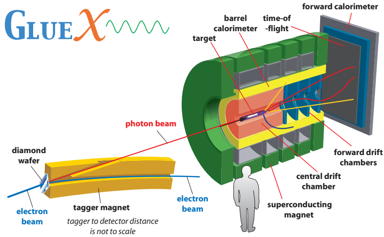
Figure 2: A schematic of the GlueX detector and beam.
