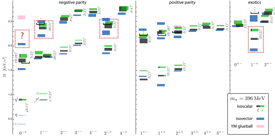
Figure 1: A compilation of recent lattice QCD computations for both the isoscalar and isovector light mesons from Ref. [2], including \ell\bar{\ell} ( |\ell\bar{\ell}\rangle \equiv (|u\bar{u}\rangle + |d\bar{d}\rangle)/\sqrt{2} ) and s\bar{s} mixing angles (indicated in degrees). The dynamical computation is carried out with two flavors of quarks, light ( \ell ) and strange ( s ). The s quark mass parameter is tuned to match physical s\bar{s} masses, while the light quark mass parameters are heavier, giving a pion mass of 396 MeV. The black brackets with upward ellipses represent regions of the spectrum where present techniques make it difficult to extract additional states. The dotted boxes indicate states that are interpreted as the lightest hybrid multiplet – the extraction of clear 0^{-+} states in this region is difficult in practice.
