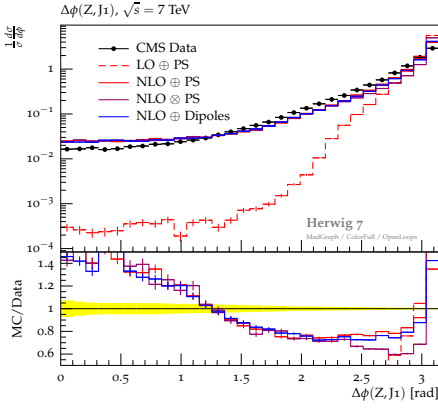
Figure 10: The distribution of separation in azimuthal angle between the Z boson and the hardest jet in Z+jets events in pp collisions at \sqrt{s} = 7 TeV in comparison with CMS data [44].
